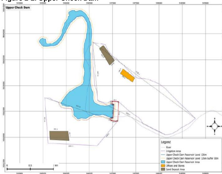
Figure 2-2. Upper Check Dam
