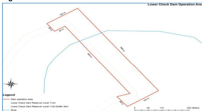
Figure 2-1. Lower Check Dam
